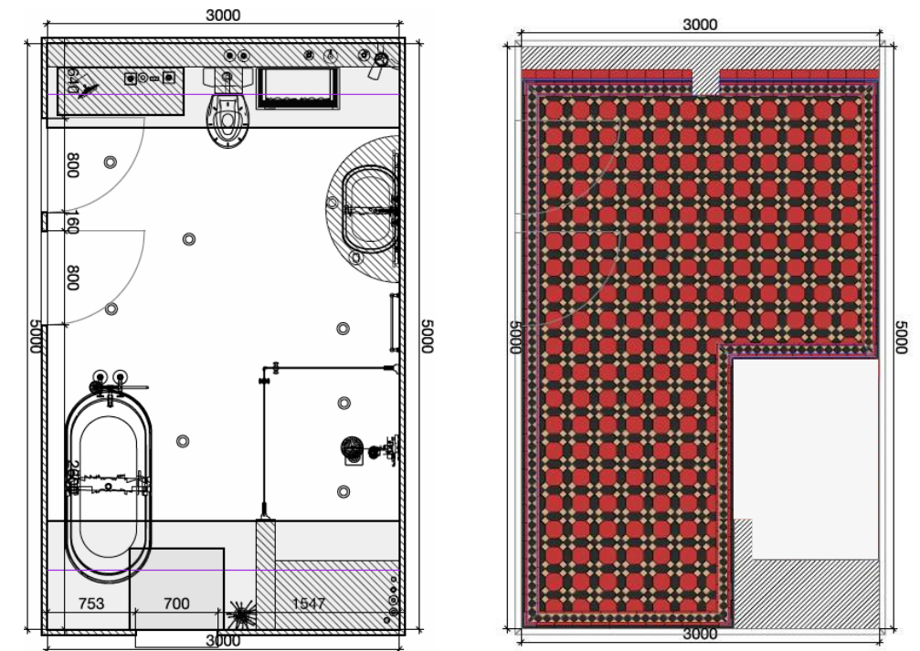
Scale floor plan and pattern layout
